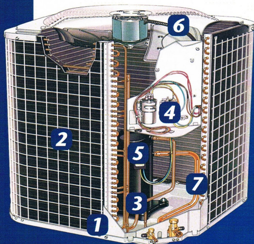
Air Conditioner
